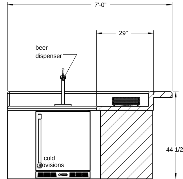
SECTION C-C
