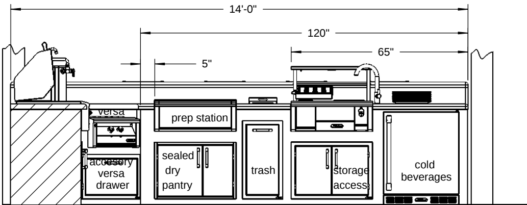
SECTION C-C
