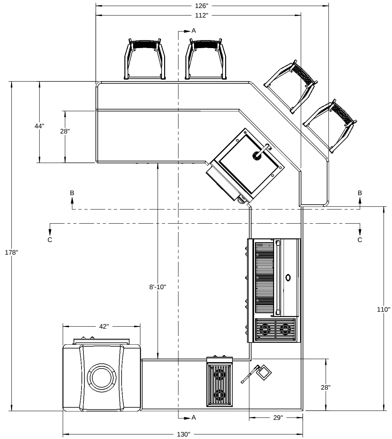
Plan View
