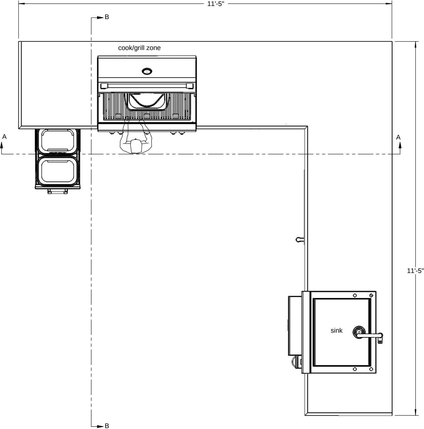
Plan View
