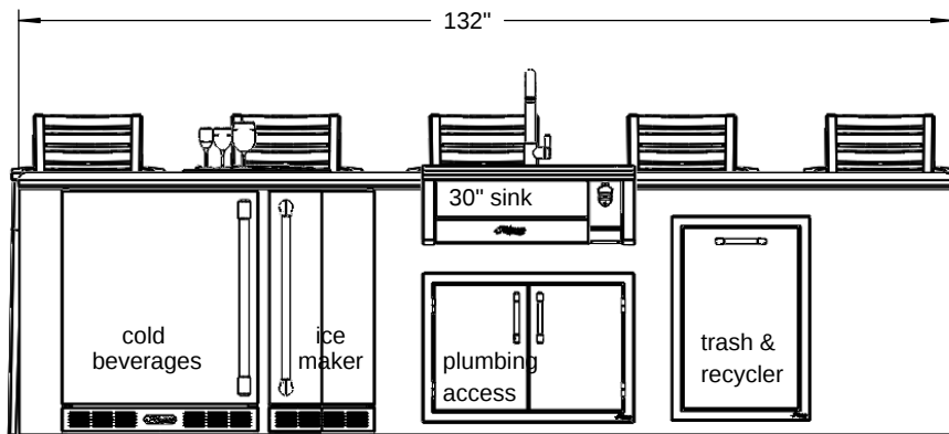
SECTION C-C
