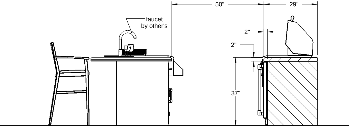
SECTION C-C
