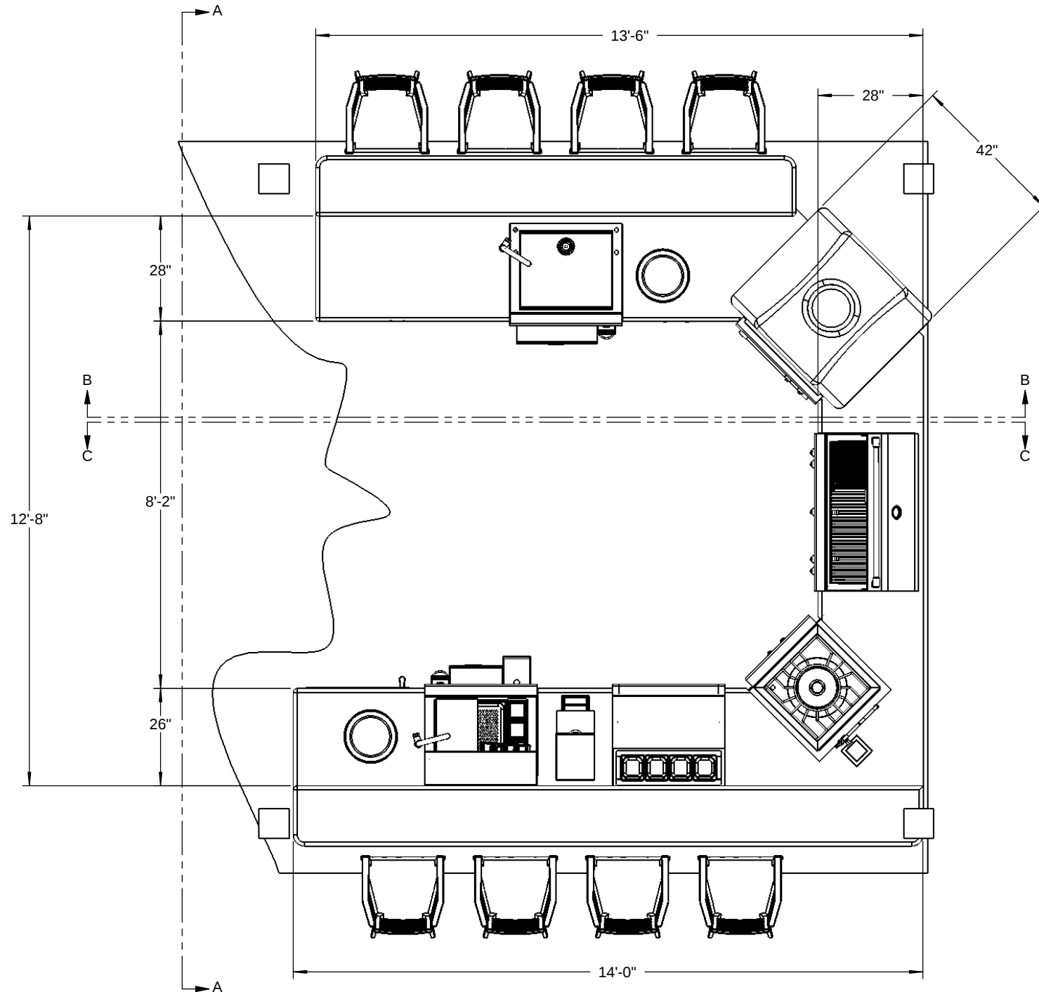
Plan View
