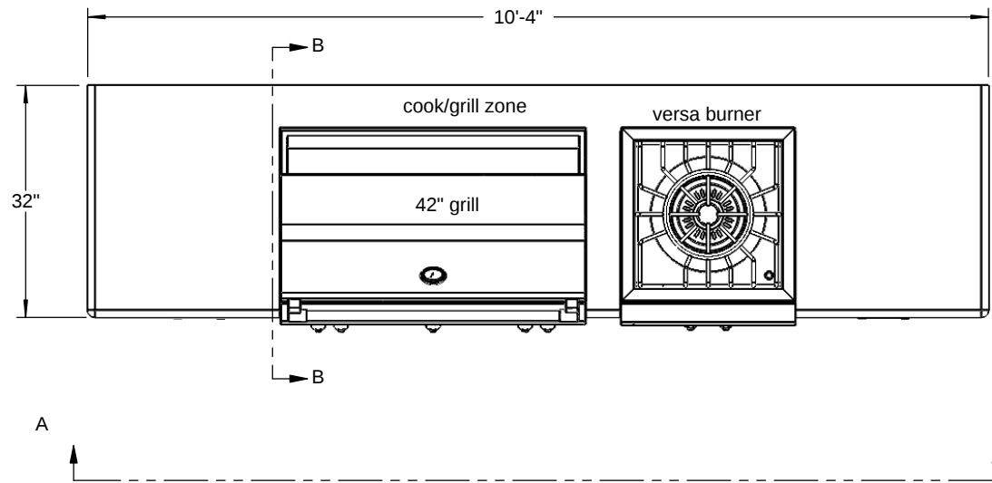
Elevation Views
